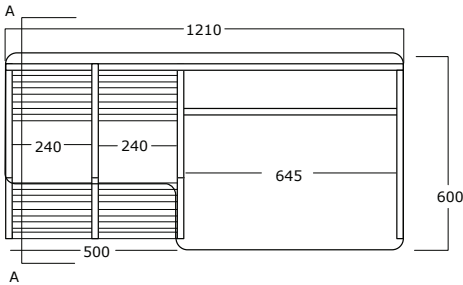
SQUARE TOP RH PLAN VIEW
