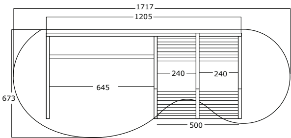
CIRCULAR TOP LH PLAN VIEW
