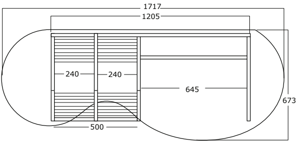
CIRCULAR TOP RH PLAN VIEW
